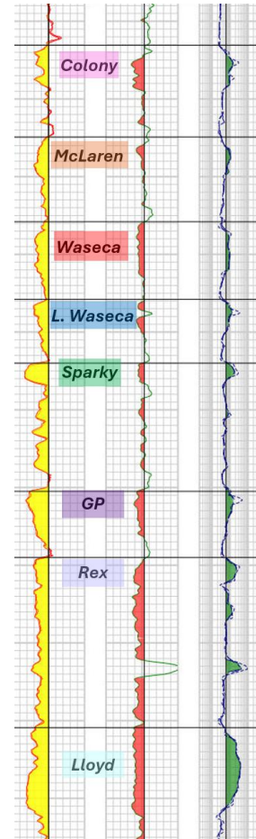
Mannville Stack - Type Log
