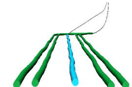
14-36 / 5-9 Pads Tuning Fork Multi-lateral with Injector in Gap
